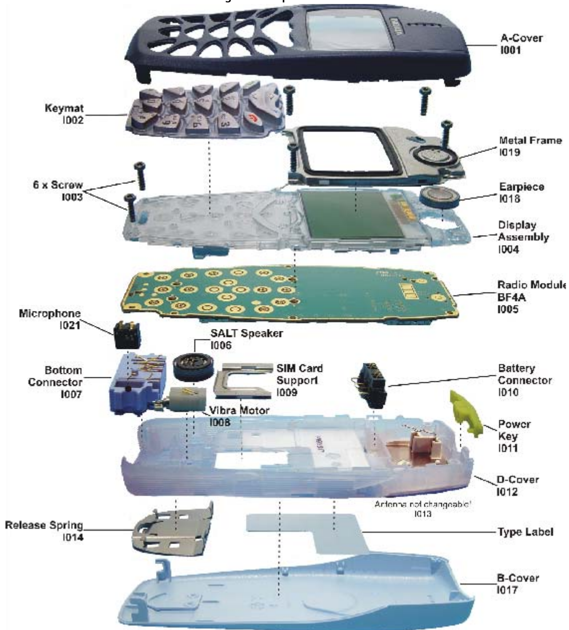
Figure 2: Exploded view of RH-9
